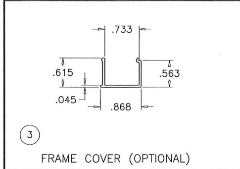
2 GLAZING STOP (OPTIONAL)
