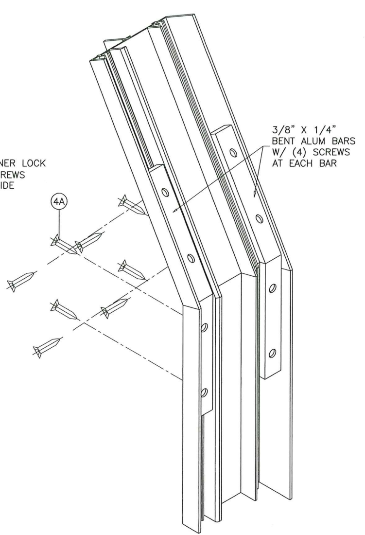
CIRCULAR OR ANGULAR WINDOWS
